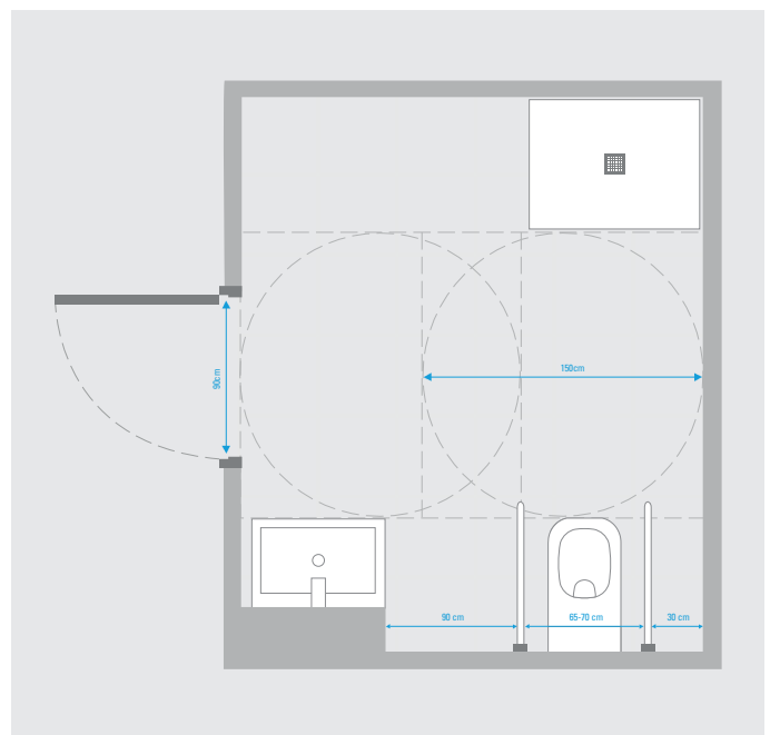
Sample layout of a wheelchair-accessible bathroom
