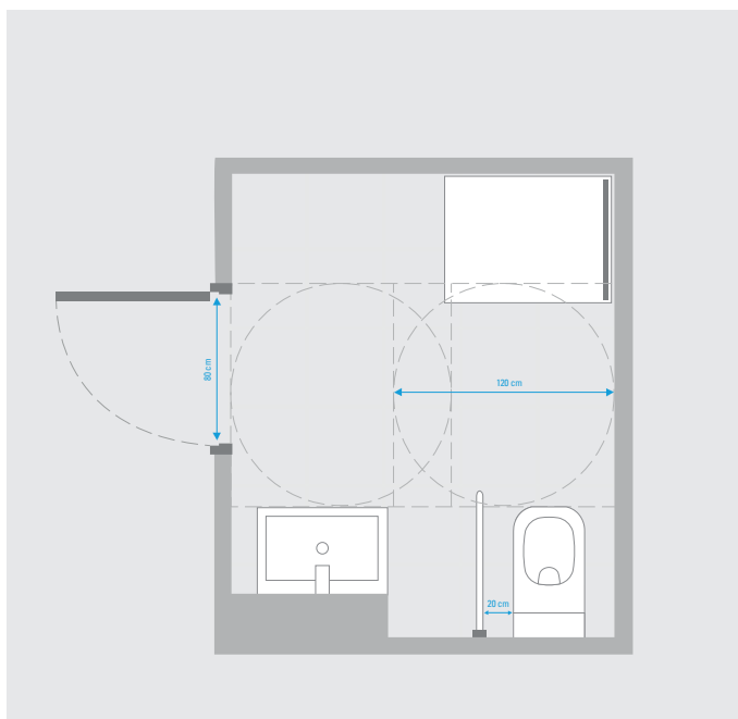
Sample layout of a barrier-free bathroom
